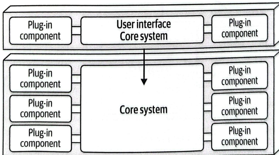
Separate user interface (multiple deployment units, both microkernel)
